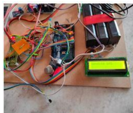
Fig14. LCD displaying SMS send using GSM
