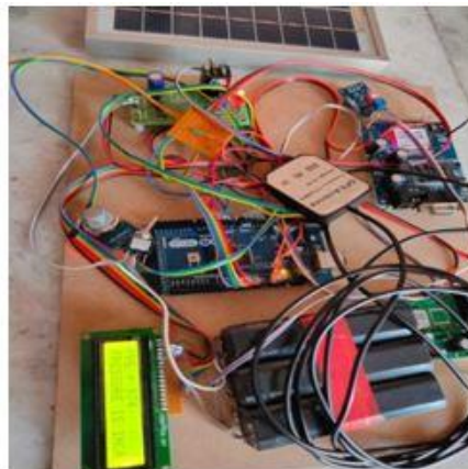
Fig13. LCD displaying Pressure is high
