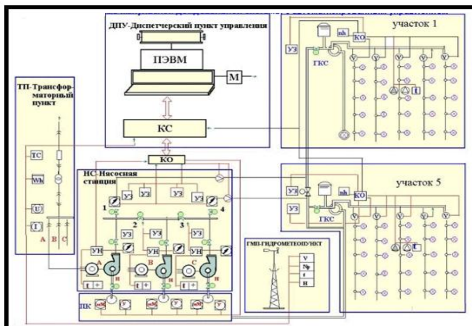
Figure2. Schematic diagram of a pulsed sprinkler automated control systems
