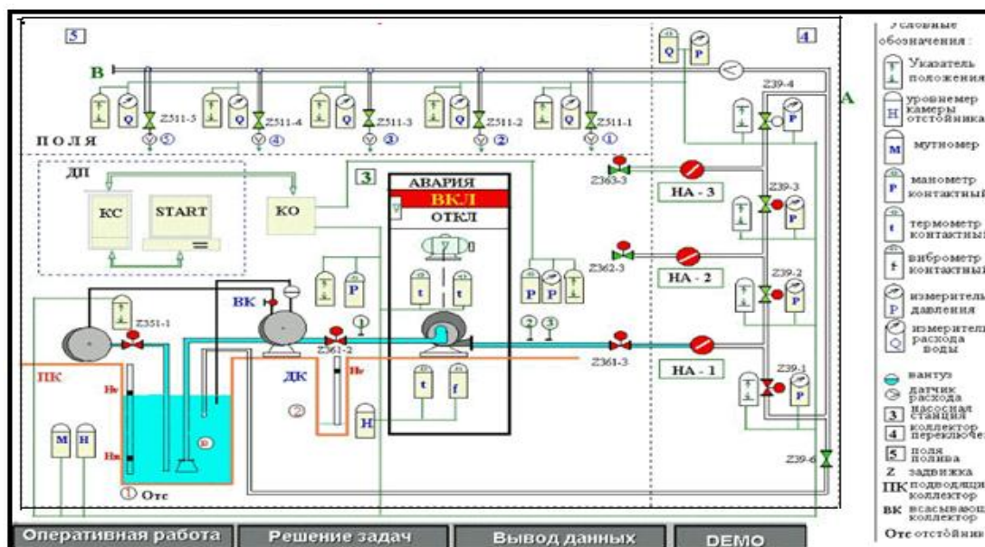
Figure3. Starting the pump motor
