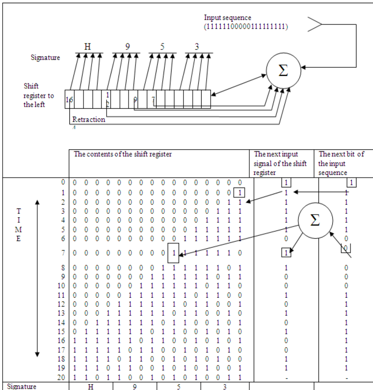
Fig4. A diagram explaining the principle of compressing an input sequence of length 20 bits by a signature analyzer.
