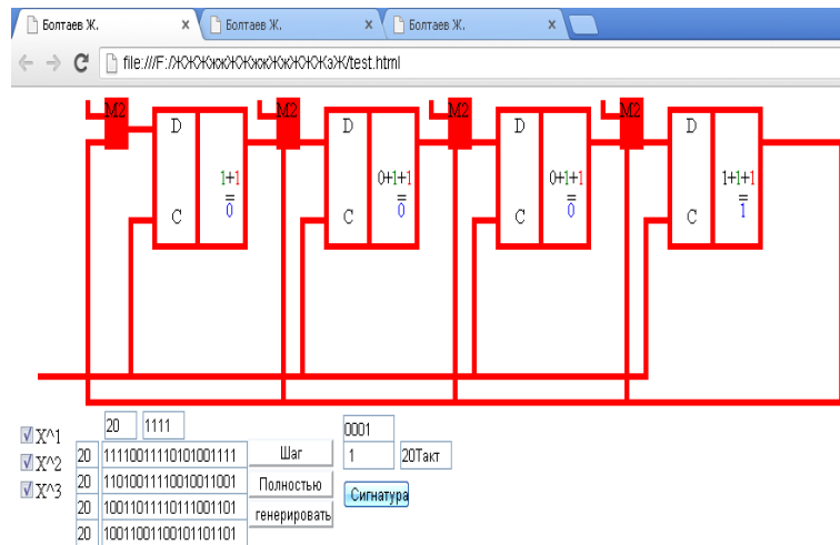
Fig10. 4-channels of the signature analyzer
