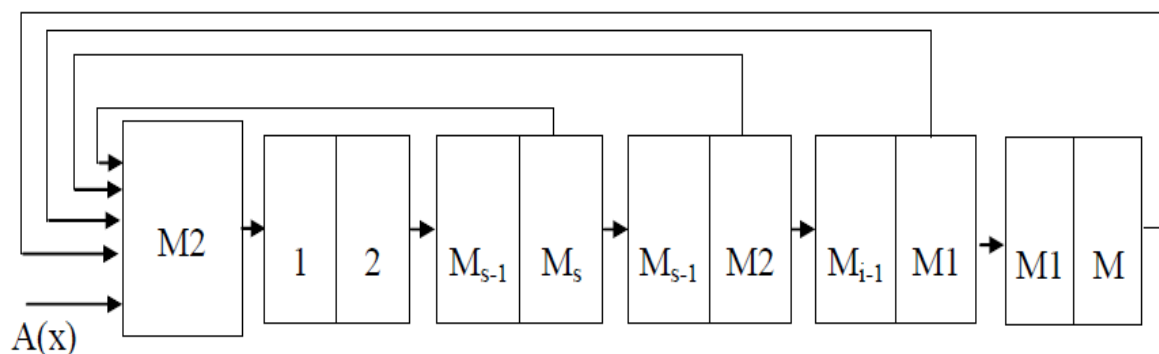
Fig3. PSG scheme based on a shift register of lengths n of digits
