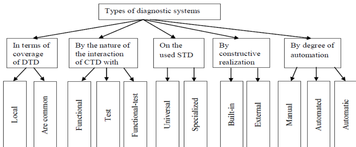
Fig2. Types of diagnostic systems
