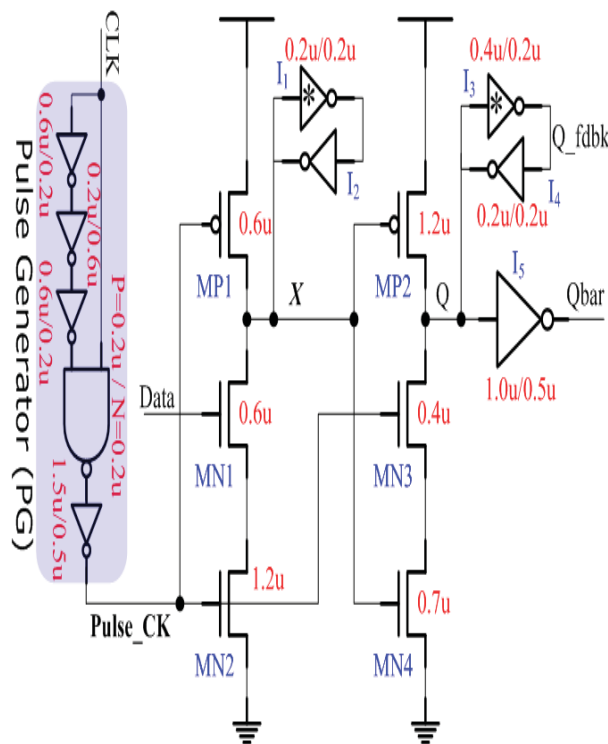
Fig.1. Conventional P-FF designs. ep-DCO [7].
