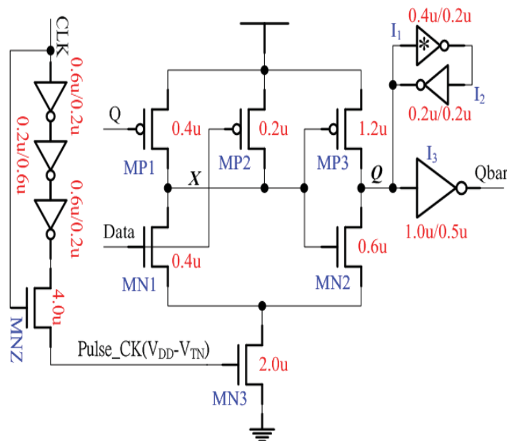
Fig.4. Conventional P-FF designs. MHLFF [19].
