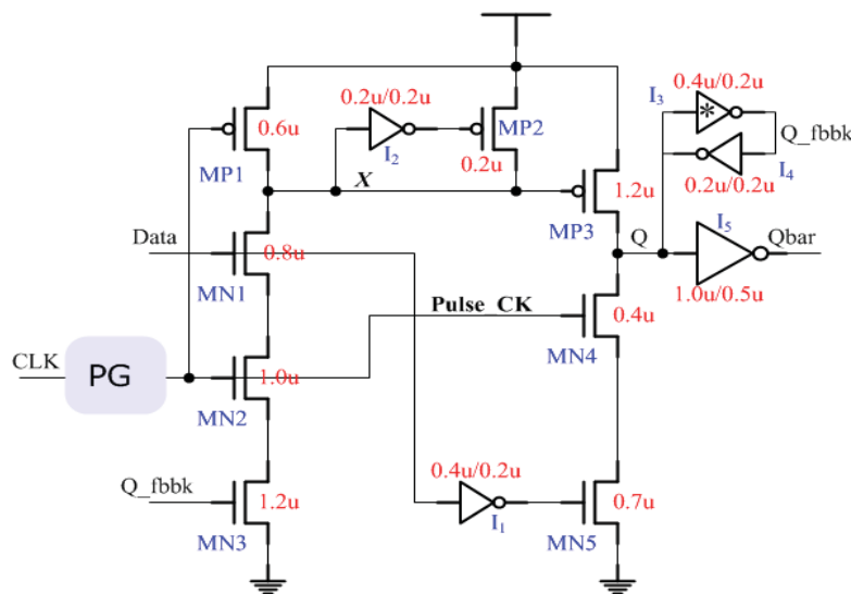
Fig.2. Conventional P-FF designs. CDFD [16].
