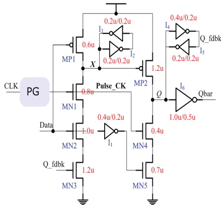
Fig.3. Conventional P-FF designs Static-CDFFF [17].
