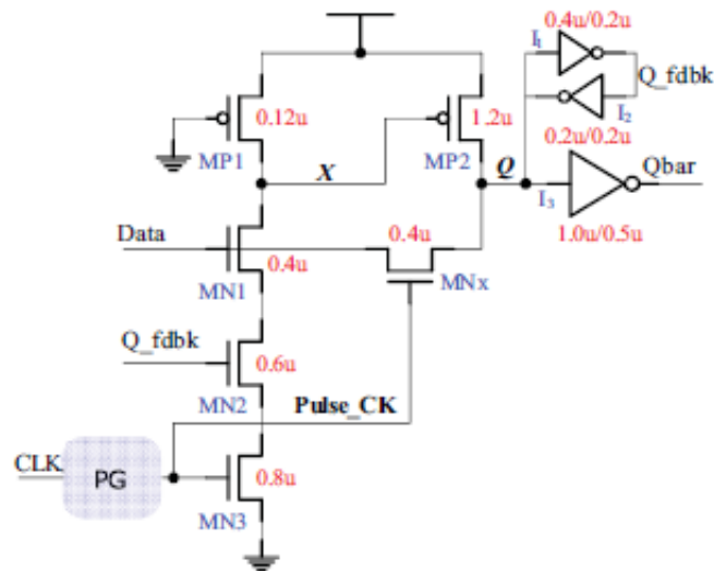
Fig.5. Schematic of the proposed P-FF design
